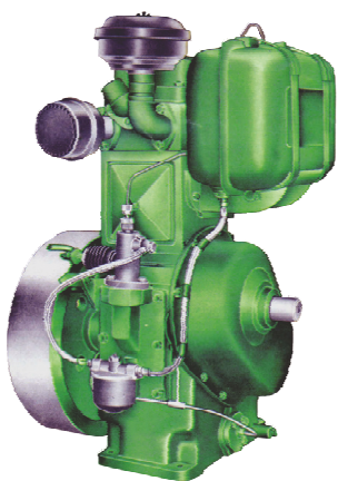
Water Cooled Diesel Engine 5 H.P. to 12.5 H.P.
