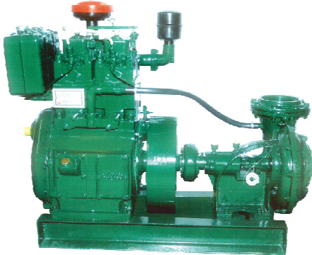
DIESEL ENGINE 16 H.P W/C DOUBLE CYLINDER WITH 6" X 6" PUMP
